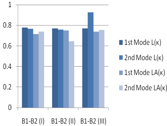
Figure 2(a): Agreement rate for B1-B2 at different iterations.
